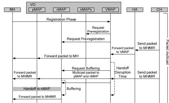
Fig. 9 Call-flow of pre-registration
