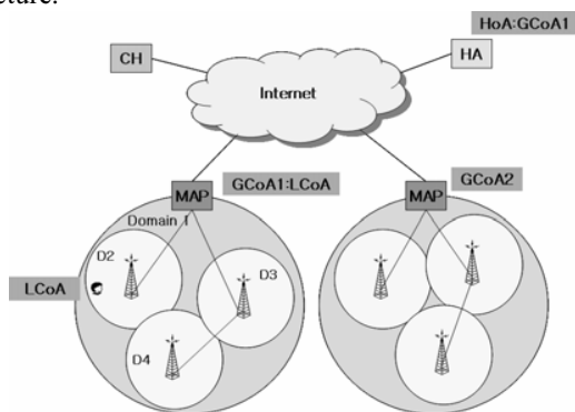
Fig. 1 N-level hierarchical mobility management architecture
