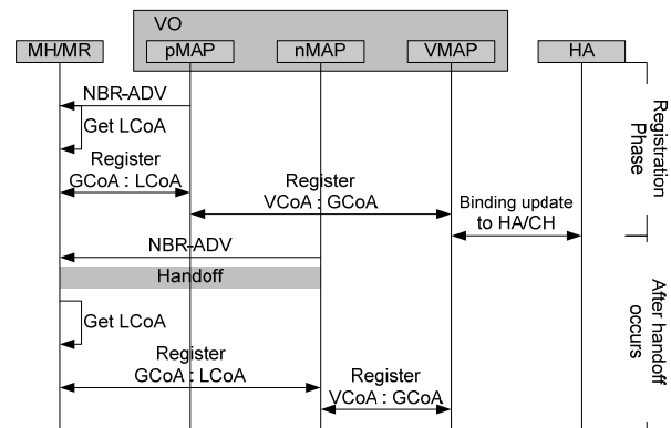
Fig. 5 Call-flow of the registration phase
