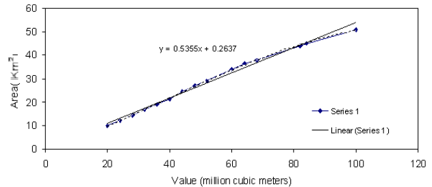
Fig. 2 Linear system of surface volume-area relations
