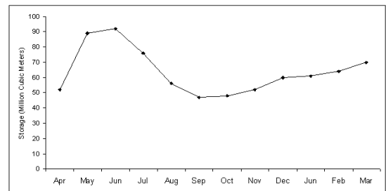
Fig. 3 Curve of reservoir exploitation of Meijaran Dam
