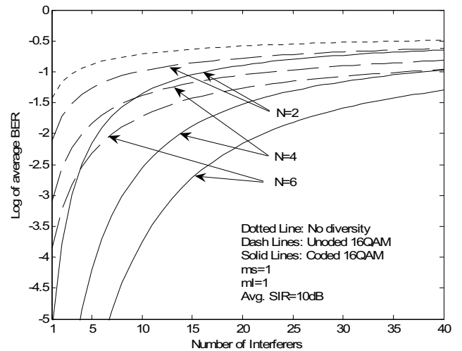
Fig. 3 The average BER versus number of interferers, L for uncoded and coded 16-QAM under N -branch MRC diversity with identical mean power interferers in a Nakagami fading environment ( m_s=1 , m_f=1 , Avg. SIR q=10 dB).
