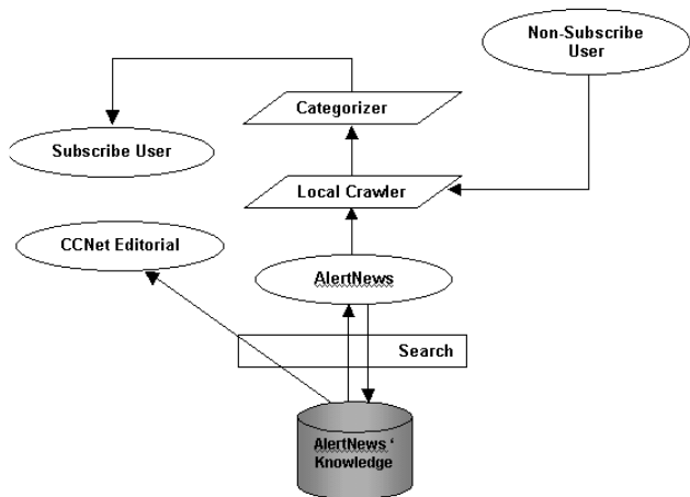
Fig. 10 AlertNews Knowledge base Model
