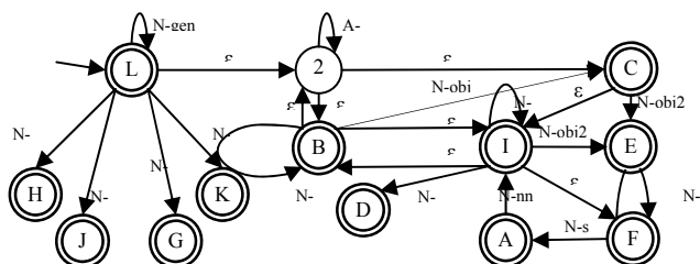
Fig. 6 Finite-state Automaton for noun phrases extraction
