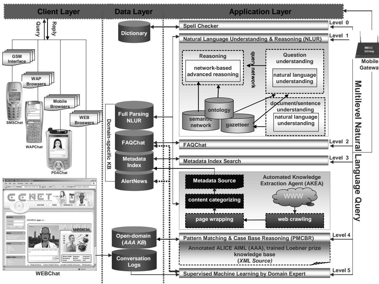
Fig. 1 AINI's Architecture in the CCNet Portal
