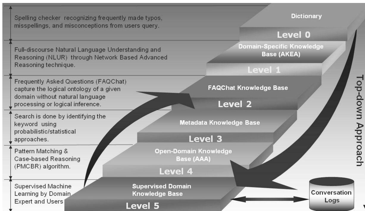
Fig. 2 Top-Down NL-Query Approach
