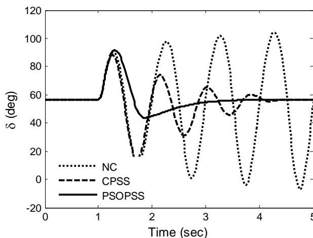
Fig. 14 Power angle response of for 3-cycle 3-phase fault disturbance at Bus 2 cleared by both line tripping with heavy loading
