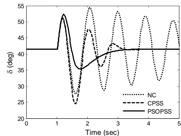
Fig. 7 Power angle response of for 3-cycle 3-phase fault disturbance at Bus 2 with nominal loading condition.
