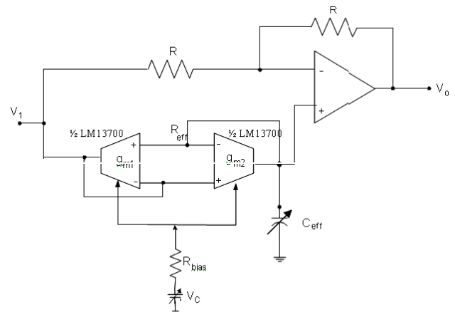
Fig. 12 Proposed modified wider tunable all pass filter.
