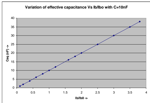
Fig. 11 Variation of effective capacitance for grounded Capacitor with I_{bias0} = 500 \mu A . I_{bias1} varied from 50 \mu A to 2 mA and C=10 nF .
