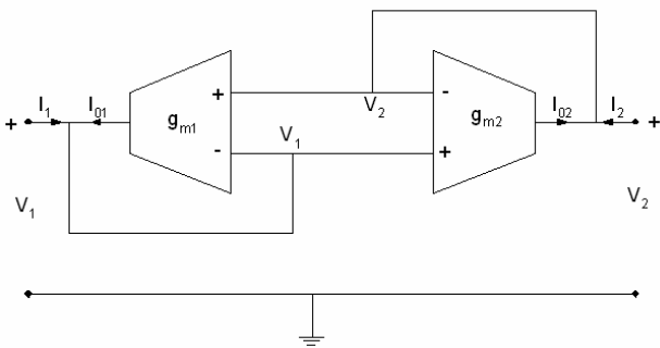
Fig. 4 Circuit for simulating floating resistor.
