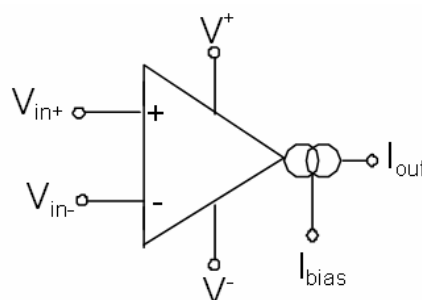
Fig. 1 Circuit symbol of OTA.
