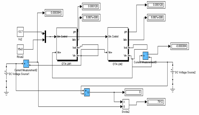
Fig. 5 Simulink model of floating resistor.
