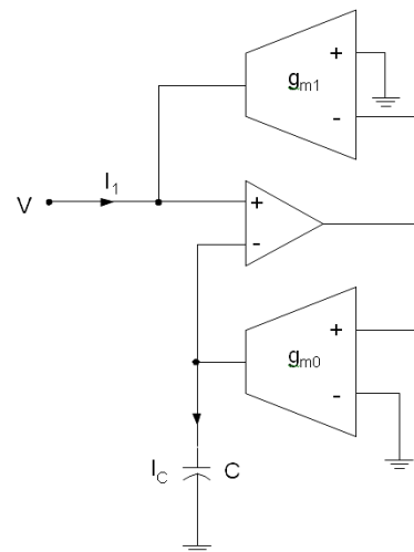
Fig. 10 Circuit for simulating grounded Capacitor.
