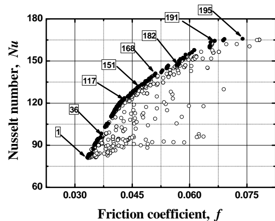
Fig. 3 Pareto sets and dominated individuals with objectives
