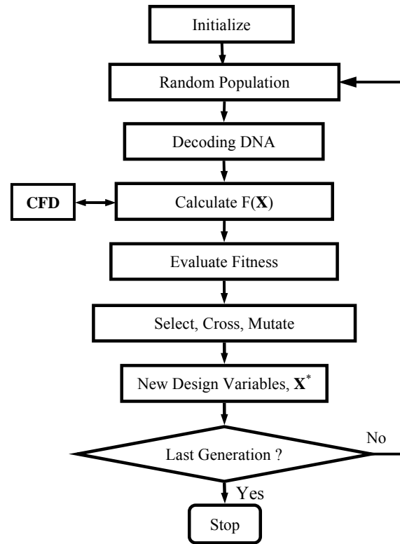
Fig. 2 Numerical procedure for optimization of internally finned tube by the genetic algorithm
