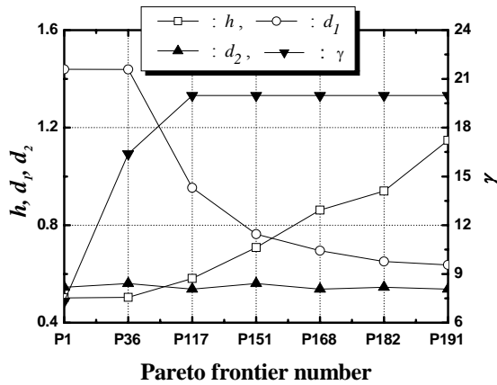
Fig. 4 Variations of design variables for Pareto individuals
