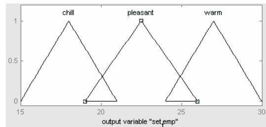
Fig. 3 Membership functions of set temperature
