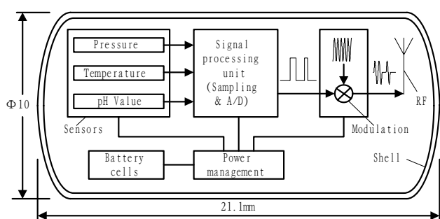
Fig.3. The schematic diagram of the telemetric capsule
