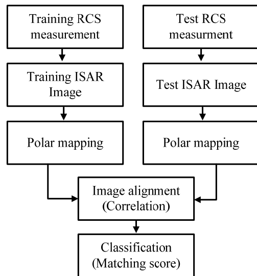
Fig. 2 Classification procedure
