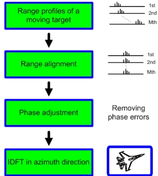
Fig. 1 Range-Doppler algorithm [4]
