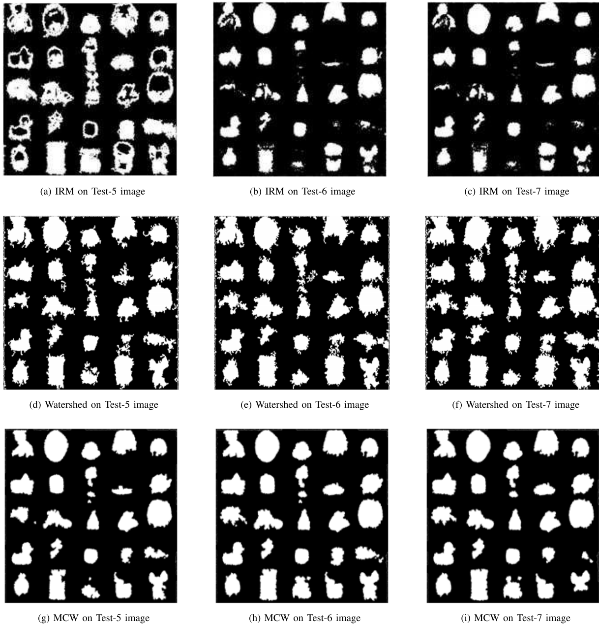
Fig. 10: Segmented output of Test-5, Test-6, Test-7 images by Integrated region matching (IRM), Watershed and Marker controlled watershed (MCW) method.
