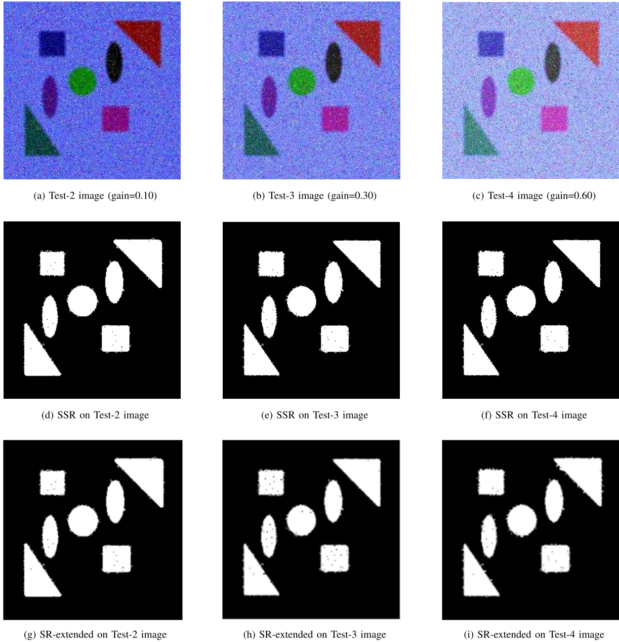
Fig. 7: Segmented output of Test-2, Test-3 and Test-4 images by proposed SSR method and SR-extended method.
