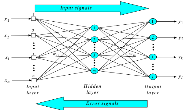
Fig. 9 Three-layer back-propagation neural network [7]
