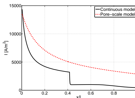
Fig. 5 Local current density distributions along the flow fields based on continuous and pore-scale models
