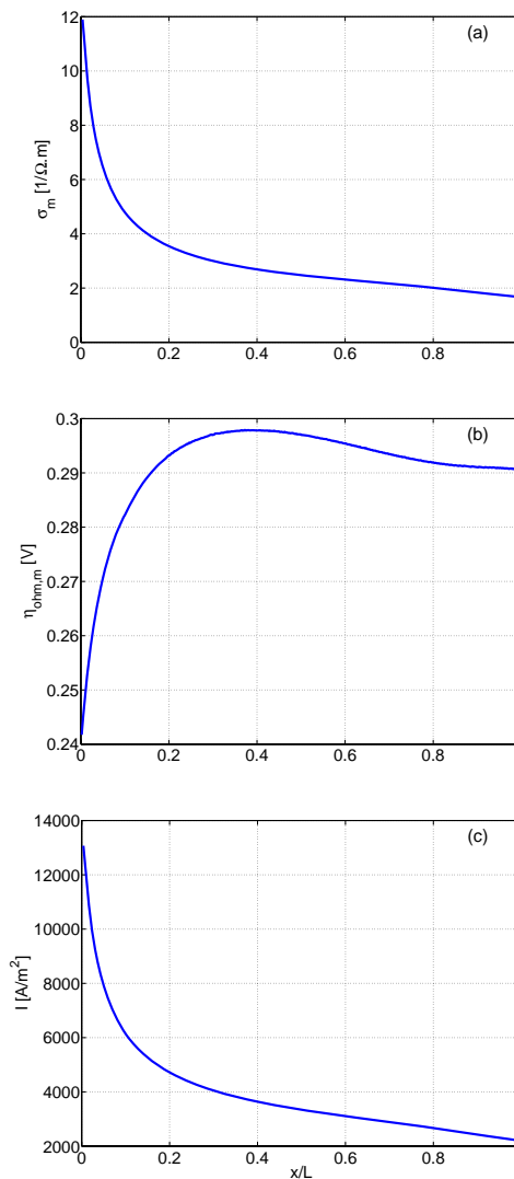
Fig. 9 Variations of (a) membrane conductivity, (b) ohmic overpotential, and (c) current density (RH c in = 85%, RH a in = 100%, S c = 1.75, S a = 1.2, P c out = 1 atm, T = 353 K)
