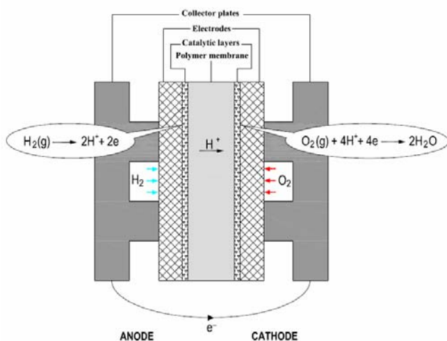
Fig. 1 Schematics of a PEM fuel cell
