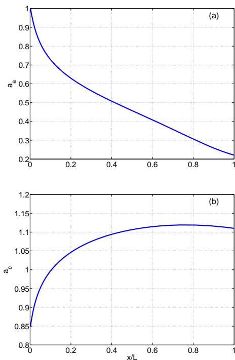
Fig. 7 Variations of (a) anode and (b) cathode water activities. (RH c in = 85%, RH a in = 100%, S c = 1.75, S a = 1.2, P c out = 1 atm, T = 353 K)
