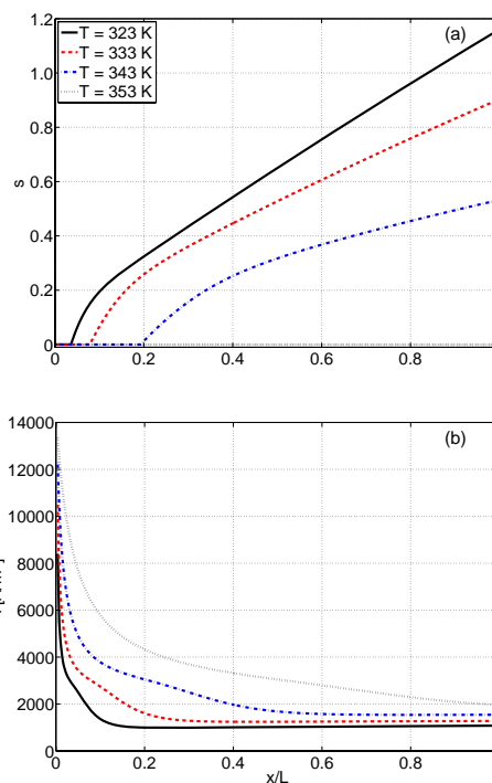
Fig. 15 Effect of cell temperature on (a) liquid water saturation and (b) local current density ( RH_c^{in} = 60\% , RH_a^{in} = 100\% , S_c = 1.75 , S_a = 1.2 , P_c^{out} = 1 atm)
