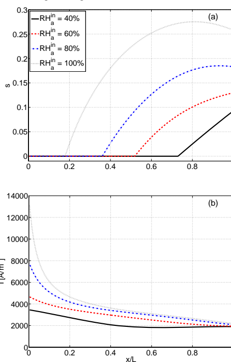
Fig. 11 Effect of anode inlet humidity on (a) liquid water saturation and (b) local current density ( RH_c^{in} = 80\% , S_c = 1.75 , S_a = 1.2 , P_c^{out} = 1 atm, T = 353 K)
