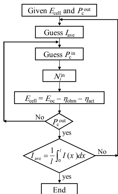
Fig. 4 Flow chart of solution procedure
