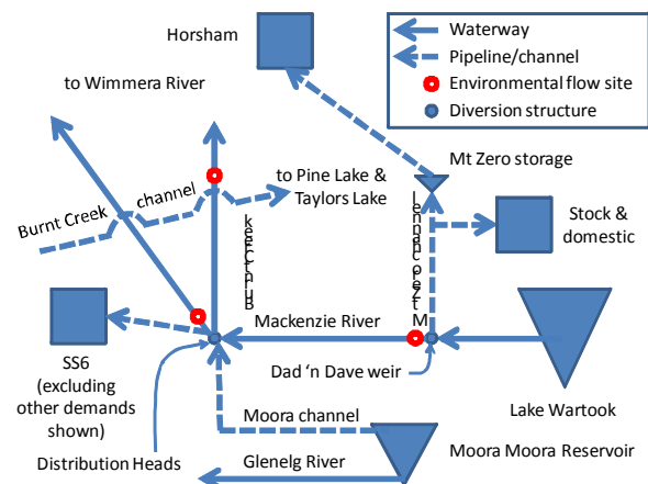
Fig. 7 Schematic representation of Supply System 6 (SS6)
