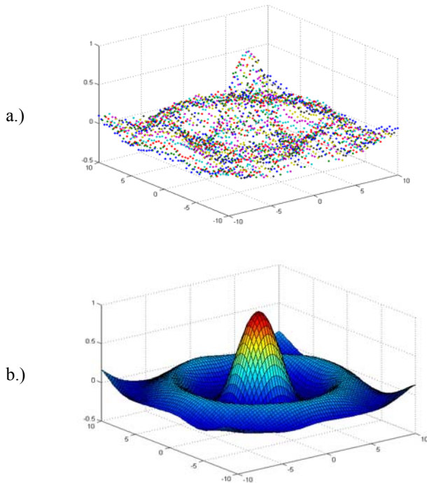
Fig. 5 Approximation of a two-dimensional sinc function. a.) The plotted training samples and b.) the result of the partially reduced LS-SVM, where the support vectors were selected by the proposed method
