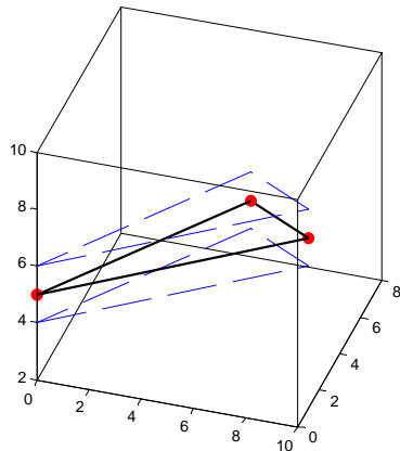
Fig. 1 The image of training samples in a kernel space of different dimensions. Using all three samples as support vectors (kernel centers), a three-dimensional kernel can space guarantees exact fit for the samples. The dashed lines represent a zone in which errors can be accepted (corresponding to the \varepsilon -insensitivity of SVM)
