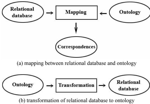
Fig. 1 Mapping vs. transformation
