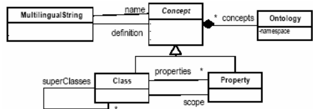
Fig. 2 Simplified ontological model
