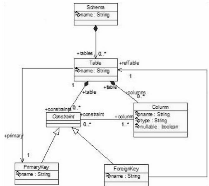
Fig. 3 Simplified relational model
