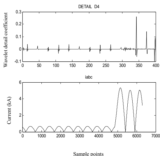
Fig. 14(b) Wavelet transient form of a-g fault
