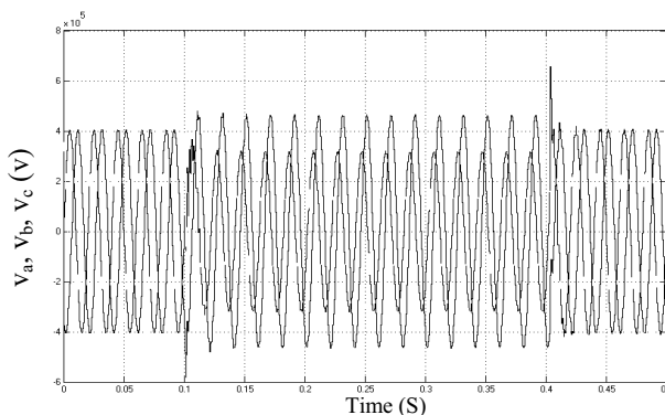
Fig. 7 Voltage waveform for double phase to ground fault (a-b-g) with R_f=40\Omega and R_g=10\Omega corresponds to the fault transition times 0.1s, 0.4s
