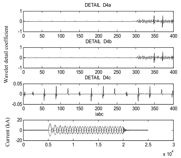
Fig. 13(a) Wavelet analysis for a-b fault
