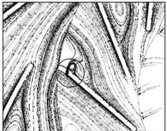
(f) Configuration M5
