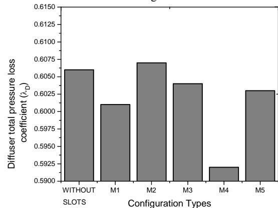
Fig. 6 Total pressure loss coefficient at the diffuser exit for the various configurations
