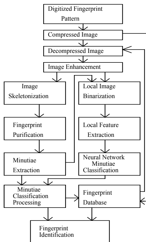
Fig. 3 Our fingerprint identification system
