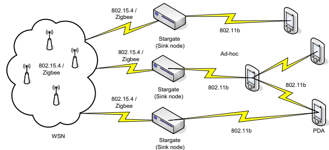
Fig. 4. Prototype layout
