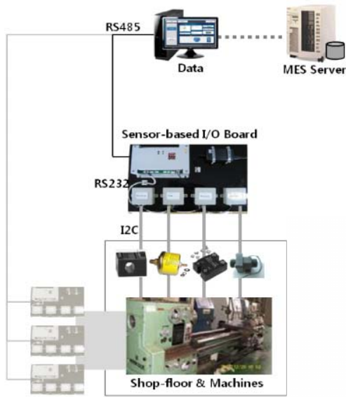
Fig. 4 Info collection using a sensor-based interface
