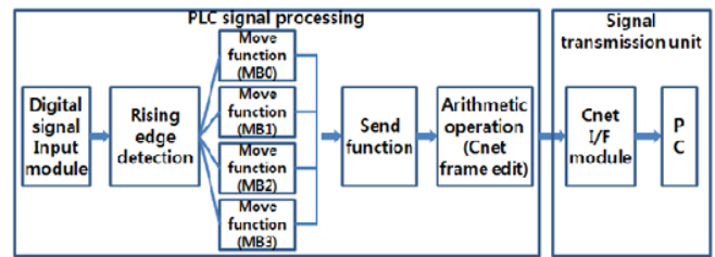
Fig. 2 Data processing using PLC
