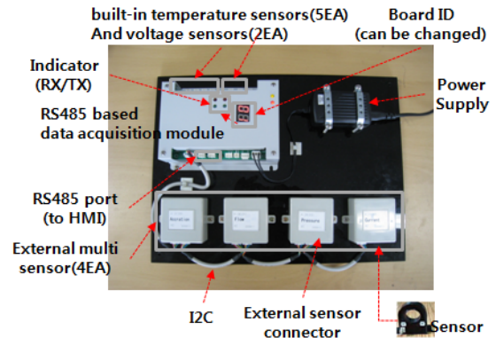
Fig. 3 Configuration of the Sensor-based interface board
