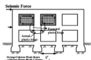
Fig. 6 Soft Story Effect
