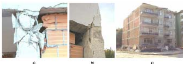
Fig. 9.Observed effects of interaction between infills and bare frame a)shear failure of column , b)exterior joint shear damage(Bonefro,Molise,2002) , c)global collapse for soft storey mechanism(Izmit,1999).
