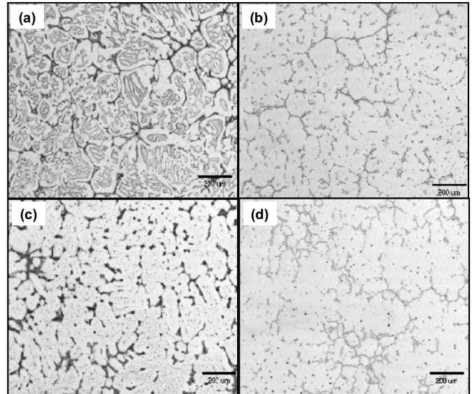
Fig. 5 Micrographs obtained after annealing the ingot No. 1 for 1 hr (a) and 64 hrs (b) and the ingot No. 2 for 1 hr (c) and 64 hrs (d) at 1230°C
