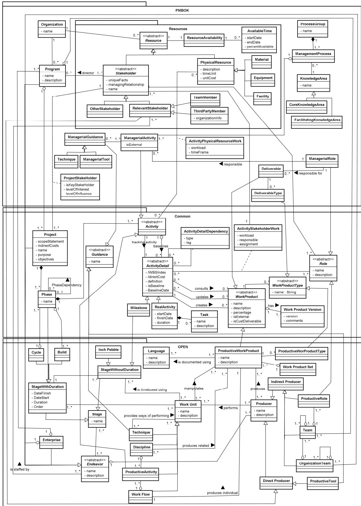
Fig. 3 PMBOK+OPEN Integrated Model
