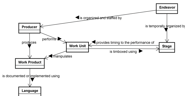
Fig. 2 Core Process Component Classes in OPEN [9]
