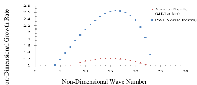
Fig. 2 Wave growth rates for different wave numbers for the annular nozzle of Li & Tankin and gas turbine nozzle of Mitra
