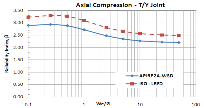
Fig. 10 T/Y – Joint Axial Compression – effect of variation in We/G on \beta
