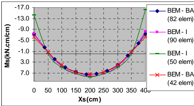
Fig. 14 Moment M_{ss} along B_4 axis
