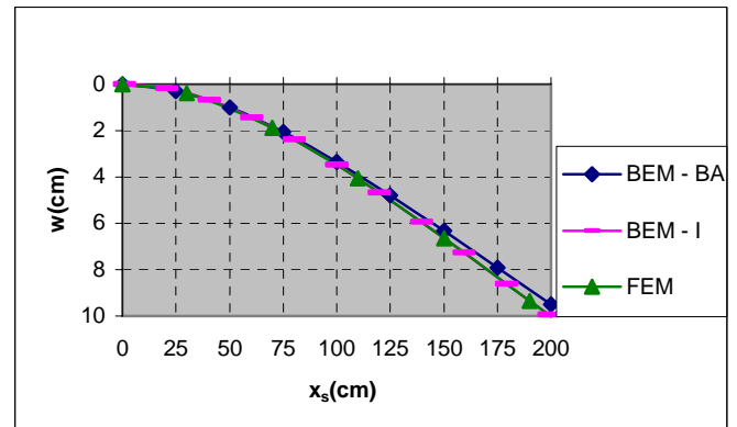
Fig. 8 Deflection along the beam axis
