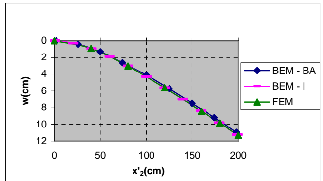
Fig. 6 Deflection in the plate, along x'_2 axis
