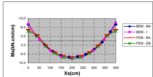
Fig. 18 Moment M_{ss} along B_4 axis
