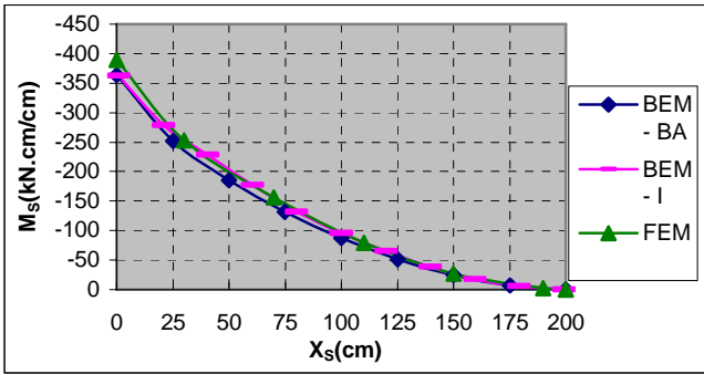
Fig. 9 Moment ( M_{22} ) along the beam axis
