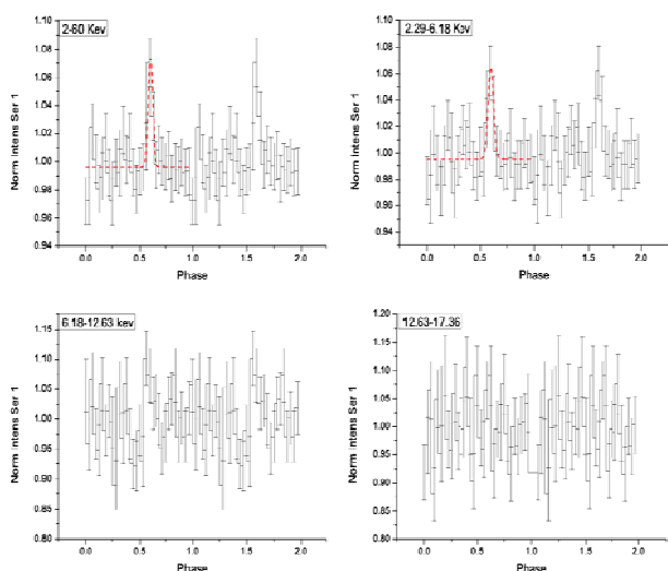
Fig. 3 Pulse profiles of PSR J0538+2817 observed by the RXTE PCA in the 2-60, 2.29-6.18,, 6.19-12.63, 12.63-17.36 keV energy window (32 bins). Two cycles are shown for clarity. The dashed lines show the best fitted Gaussian curve
