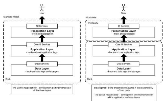
Fig. 1 Front-end application outsourcing model [authors]
