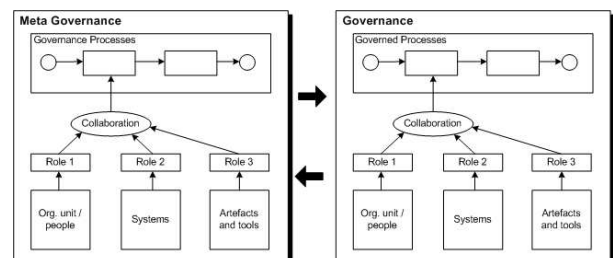
Fig. 4 Meta Governance and Governance Layers [authors]
