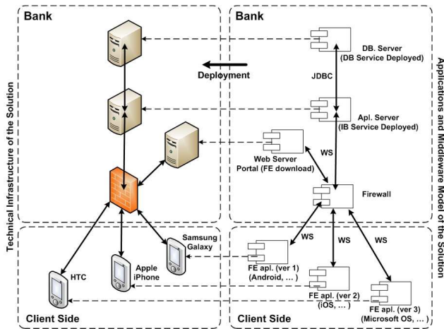
Fig. 2 Integration and Deployment Model [authors]
