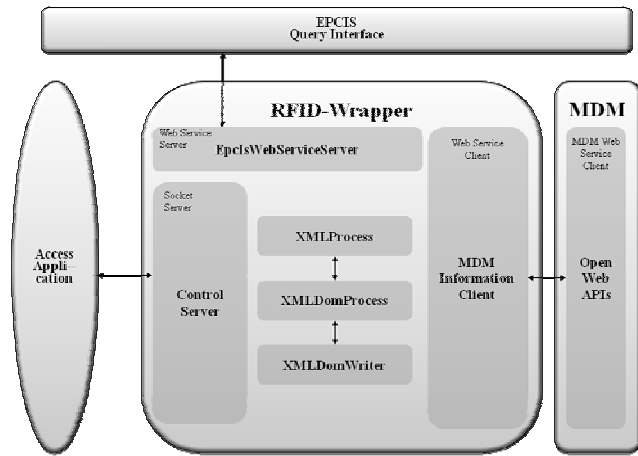
Fig. 2 Modular Structure of RFID-Wrapper
