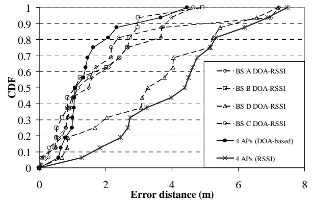
Fig. 14 Comparison between the hybrid DOA-RSSI, DOA and RSSI methods in the seminar room.
