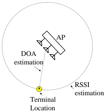
Fig. 8 Hybrid DOA-RSSI location estimation
