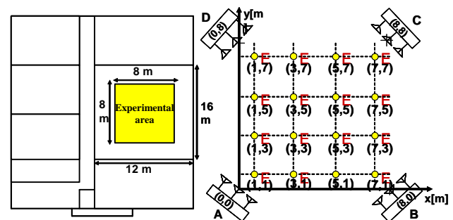
Fig. 4 Typical LOS office environment and experimental setup.
