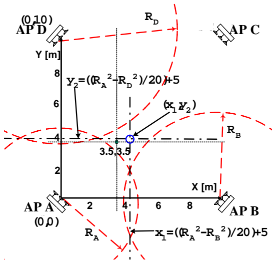
Fig. 7 RSSI-based estimation for AP AB-DA
