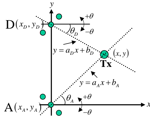
Fig. 6 The location estimation method.
