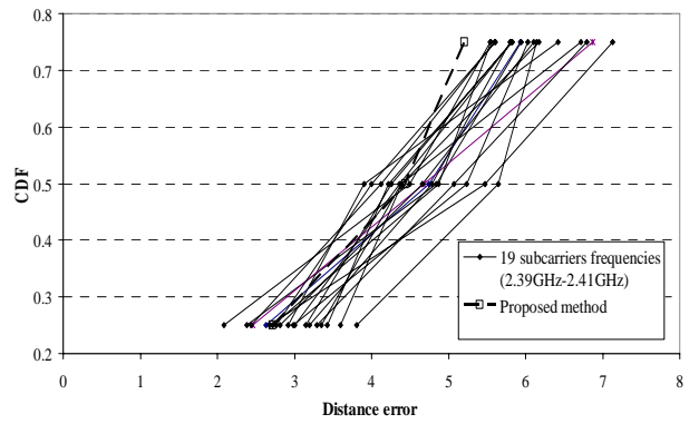
Fig. 12 Comparison of our proposed RSSI location estimation method (multiple subcarriers) to other 19 subcarriers (narrowband) at seminar room
