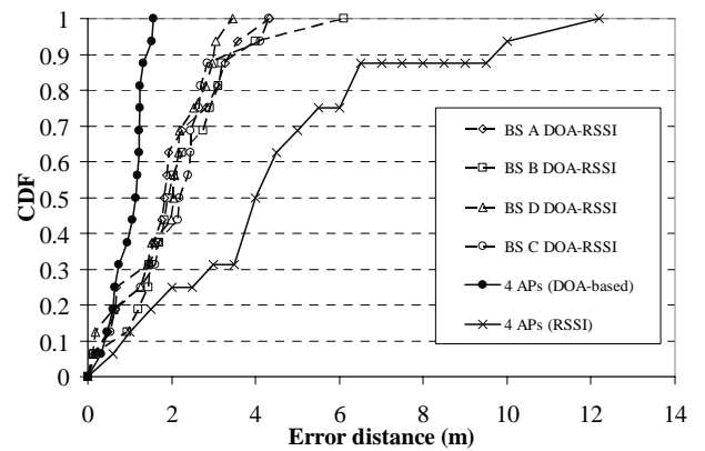
Fig. 13 Comparison between the hybrid DOA-RSSI, DOA and RSSI methods in the gymnasium hall.
