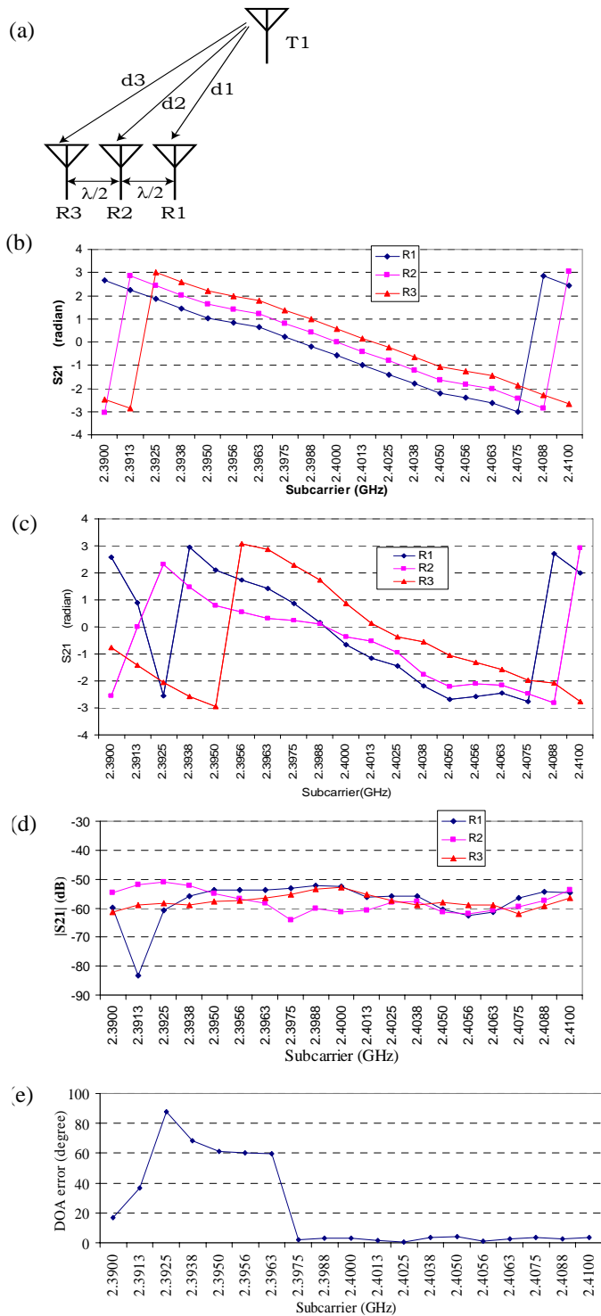
Fig. 5 DOA estimation error for each subcarrier from one sample location (Tx. coordinate=(9.5,6.5) and AP A). (a) receiving array structure (b) and (c) simulation and experimental data of received signal (d)S21 parameter (e) DOA estimation error
