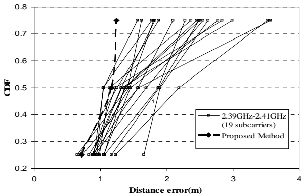
Fig. 9 Comparison of our proposed DOA location estimation method (multiple subcarriers) to other 19 subcarriers (narrowband) at Gymnasium hall
