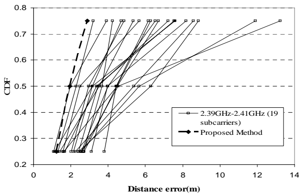
Fig. 10 Comparison of our proposed DOA location estimation method (multiple subcarriers) to other 19 subcarriers (narrowband) at seminar room
