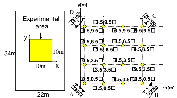
Fig. 3 The gymnasium layout and 4 APs with 16 location points.
