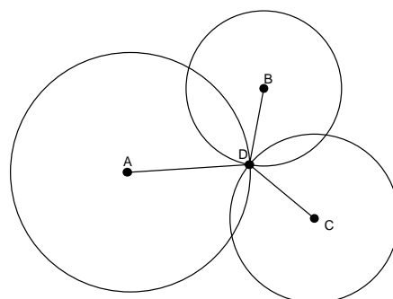
Fig. 1 Location estimation using intersecting circles from distance measurement. By calculating RSSI from D at AP A, AP B and AP C, location of terminal D can be triangulated.
