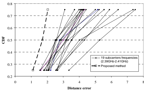
Fig. 11 Comparison of our proposed RSSI location estimation method (multiple subcarriers) to other 19 subcarriers (narrowband) at Gymnasium hall
