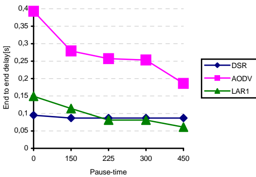
Fig. 11 End to end delay (n=1000, TL=1S)
