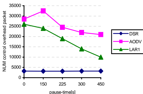
Fig. 17 Routing overhead (n=500, TL=10S)
