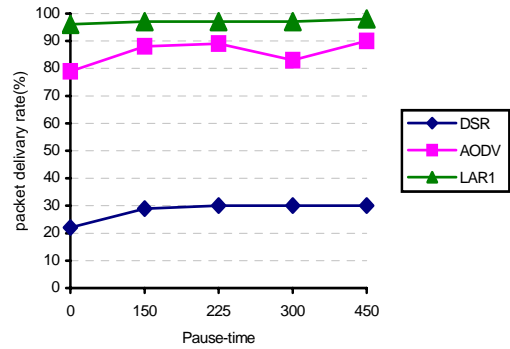
Fig. 5 Packet delivery (n=1000, TL=1S)
