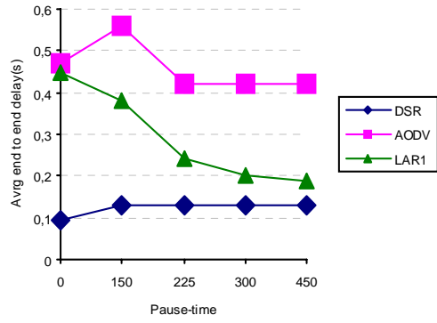
Fig. 12 End to end delay (n=1000, TL=10S)
