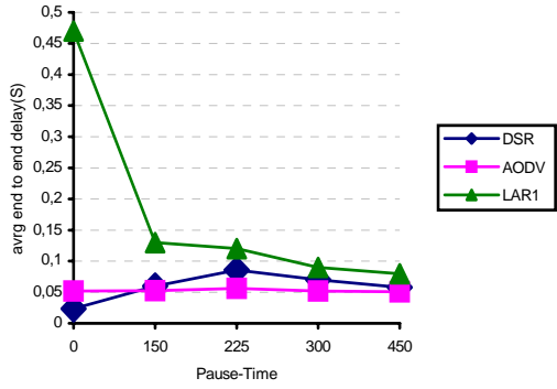
Fig. 9 End to end delay (n=100, TL=1S)
