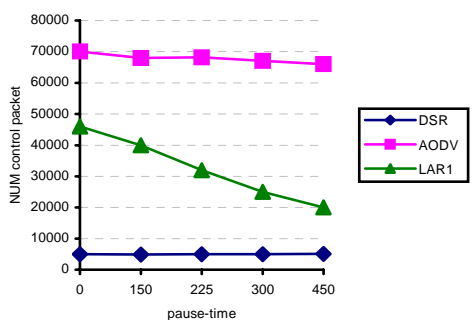
Fig. 16 Routing overhead (n=1000, TL=10S)
