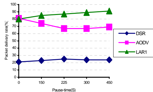
Fig. 7 Packet delivery (n=500, TL=10S)
