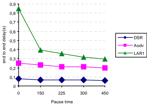
Fig. 10 End to end delay (n=100, TL=10S)
