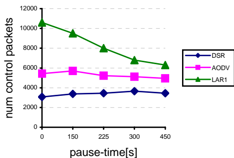
Fig. 15 Routing overhead (n=100, TL=1S)
