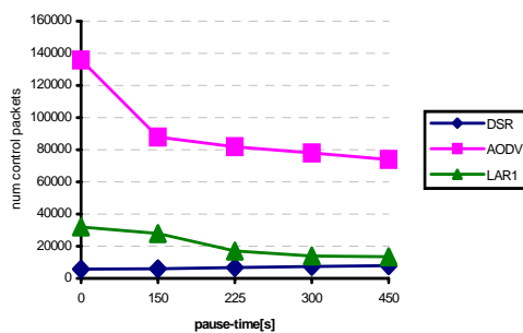
Fig. 19 Routing overhead (n=500, TL=1S)
