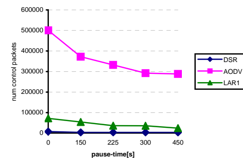
Fig. 18 Routing overhead (n=1000, TL=1S)
