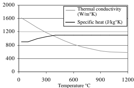
Fig. 5 Thermal properties of concrete
