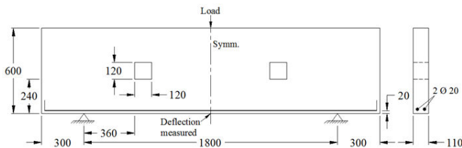
Fig. 6 Beam S05-80-3 [12]
