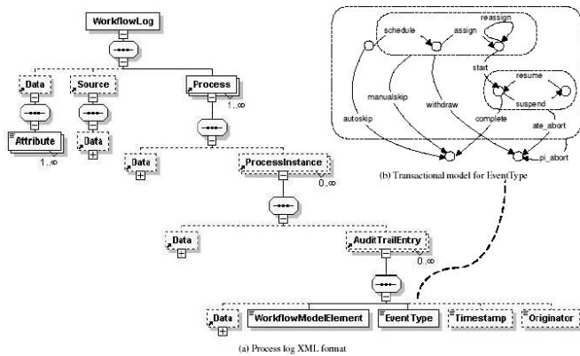
Fig. 3 Schema of the MXML format
