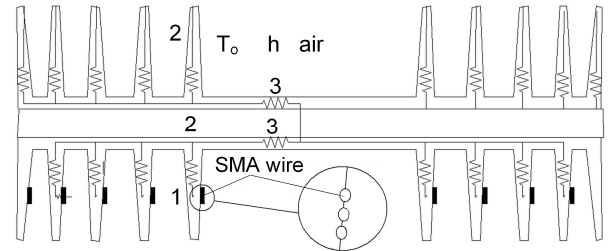
Fig. 3 Distribution of thermal resistances on the cooling system
