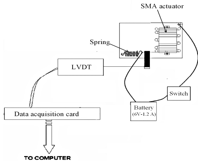
Fig. 5 Layout of the experimental setup
