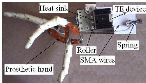
Fig. 4 Prototype for actuating one hand prostheses finger
