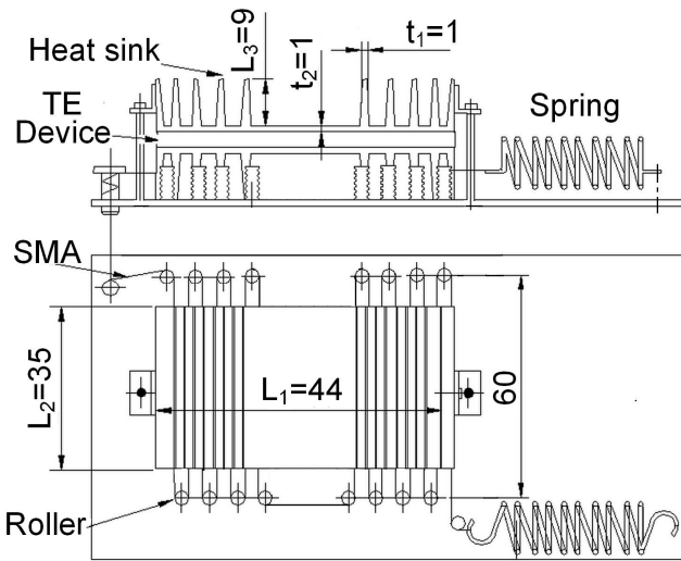
Fig. 1 Compact actuator and cooling system module
