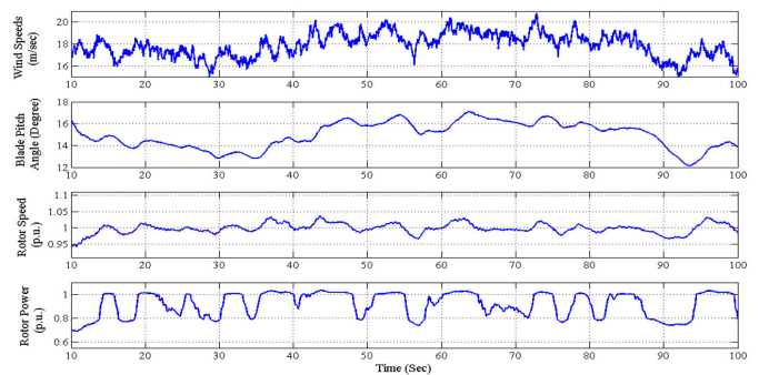
Fig. 15 Pitch angle response for stochastic wind speeds
