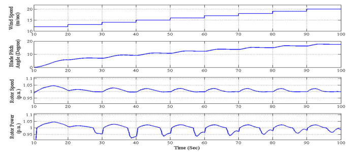
Fig. 14 Pitch angle response for step changes in wind speeds
