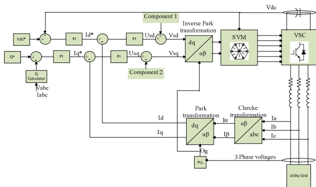
Fig. 13 Grid Side Converter Control
