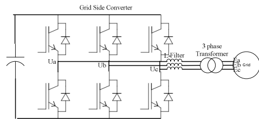
Fig. 9 Grid Side Converter
