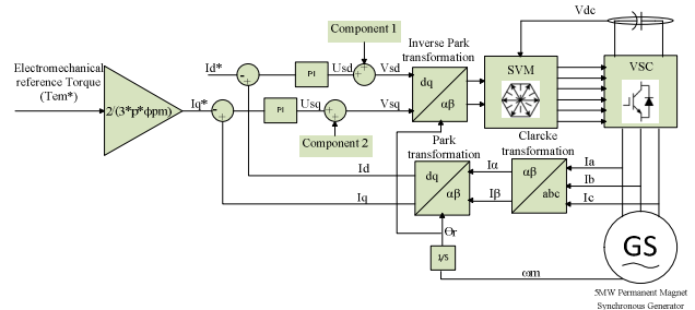
Fig. 11 Generator Side Control
