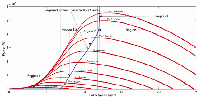
Fig. 10 Power curve for wind turbine
