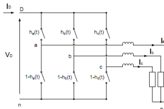
Fig. 8 Equivalent circuit of voltage source converter with ideal switch
