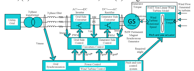
Fig. 1 Block diagram of wind turbine system
