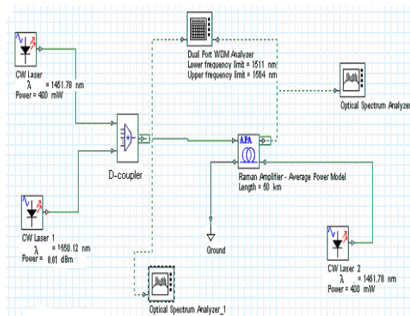
Fig. 2 The simulation layout, bidirectional pumping
