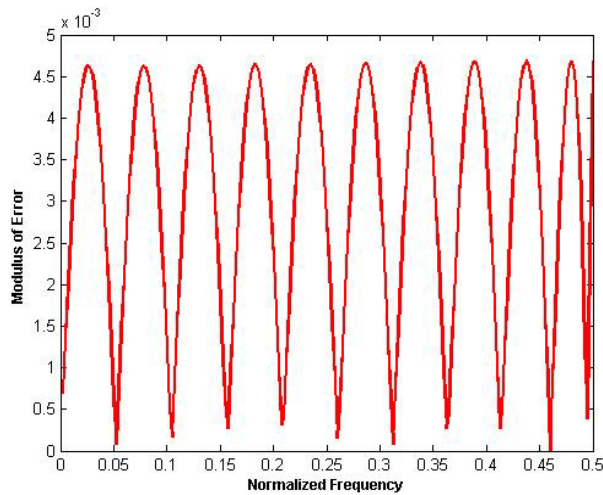
(b) Equiripple error distribution
