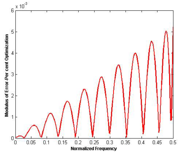
(b) Optimized modulus of absolute error
