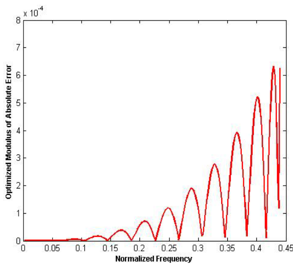
(c) Optimized modulus of absolute error
