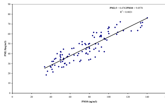
Fig. 3 Correlation between PM10 and PM2.5 during the study period
