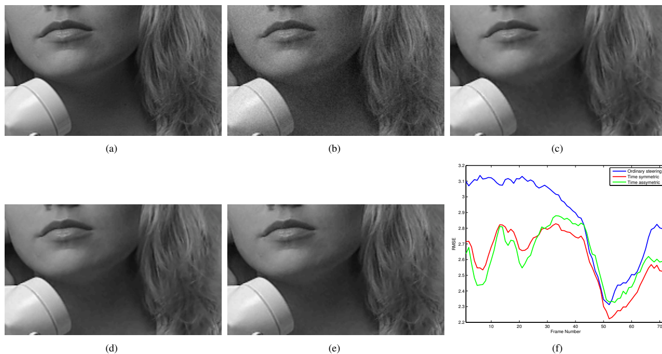
Fig. 5. Detail of frame number 7 of, (a) the original frame and, (b) the frame with added noise with N(0, 5) . The resulting frame of filtering with the, (c) steering kernel of size [5 \times 5] , (d) video steering kernel of size [5 \times 5 \times 3] and (e) video steering kernel of size [5 \times 5 \times 3] and (f) The frame by frame comparison of the RMSE of the three methods.
