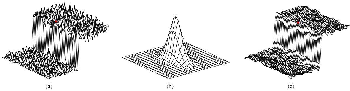
Fig. 2. Construction of the steering kernel based on the red dot in (a) in a 21x21 neighborhood. (b) The steering kernel based on the structure of the gradients. (c) The result of filtering with the steering kernel with parameter \alpha_s = 11 .
