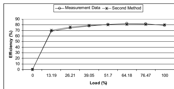
Fig. 3. Measured and estimated efficiency versus load in the second method, for the first motor
