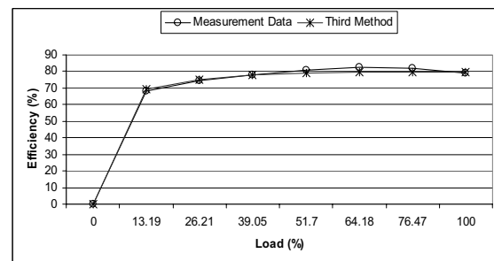
Fig. 4. Measured and estimated efficiency versus load in the third method, for the first motor
