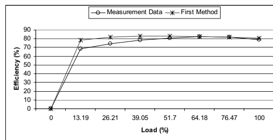
Fig. 2. Measured and estimated efficiency versus load in the first method, for the first motor
