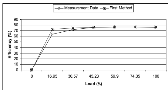
Fig. 6. Measured o and estimated * efficiency versus load in the first method, for the second motor
