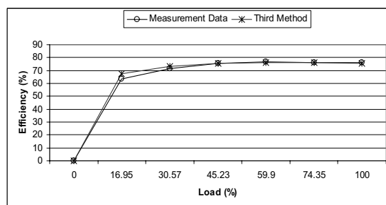
Fig. 8. Measured o and estimated * efficiency versus load in the third method, for the second motor
