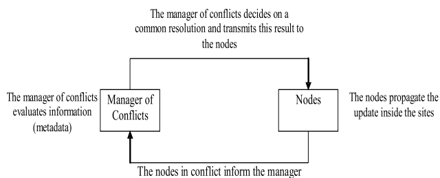
Fig. 3. Process of resolution of conflicts
