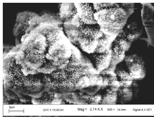
Fig. 1c SEM image of schwertmannite
