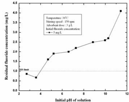
Fig. 4 pH effect of fluoride adsorption on schwertmannite
