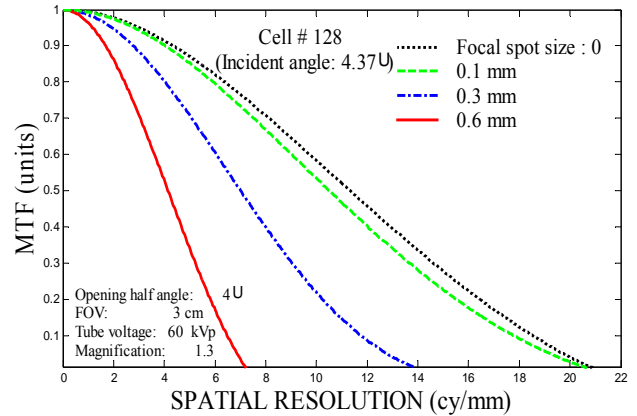
Fig. 4 At opening half angle of 4^\circ , the focal spot sizes of 0.6 mm and 0.3 mm greatly limit the spatial resolution of the system.
