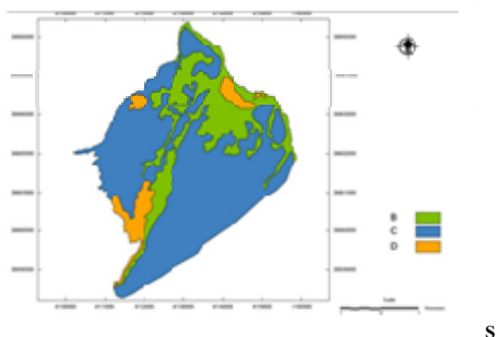
Fig. 2 The map of soil hydrological groups
