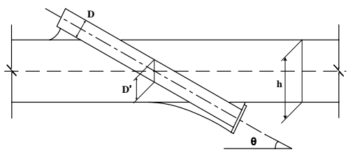
Fig. 7 Outer-diameter limit of the fixing pipe
