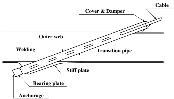
Fig. 2 Detailed drawing of the fixing pipe
