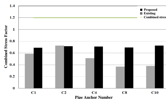
Fig. 12 Comparison of the composite stresses of the fixing pipe
