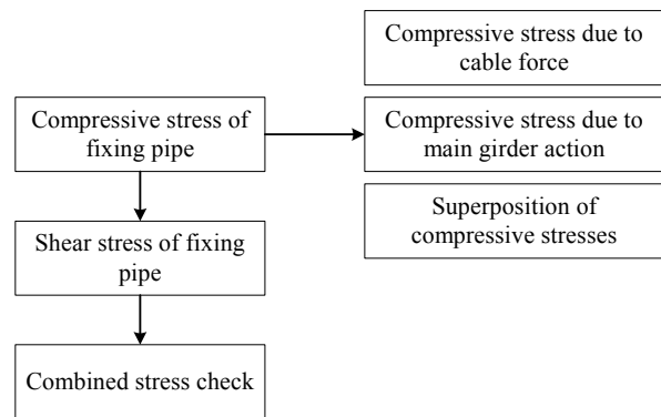
Fig. 3 Existing design of the fixing pipe
