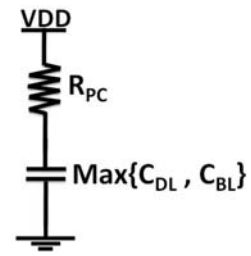
(a) RC Network During Pre-charging
