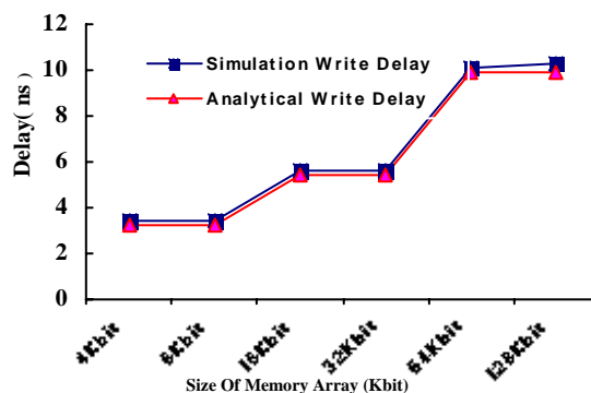
Fig. 7 Simulation and analytical write delay
