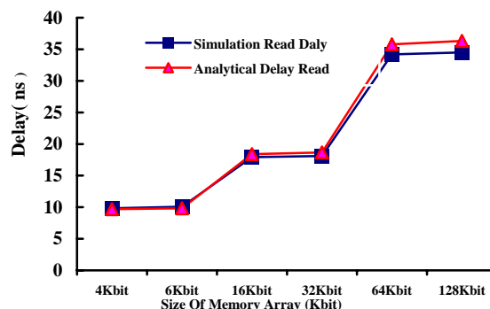
Fig. 6 Simulation and analytical read delay
