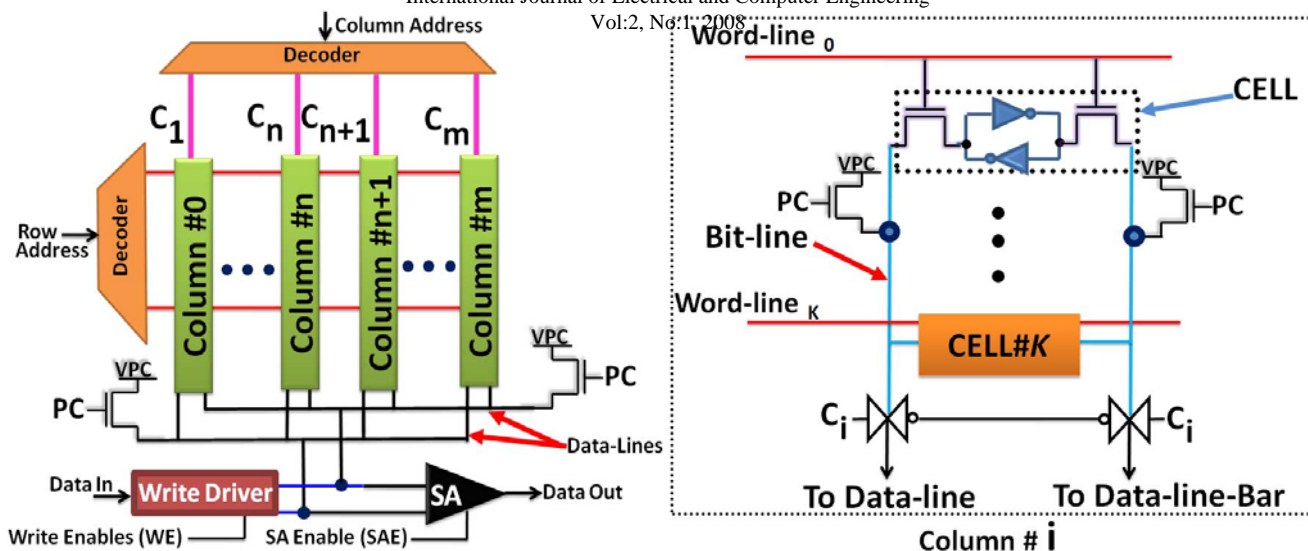
Fig. 1 Structure of conventional SRAM
