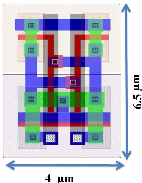
Fig. 3 Conventional layout of 6 transistor SRAM cell
