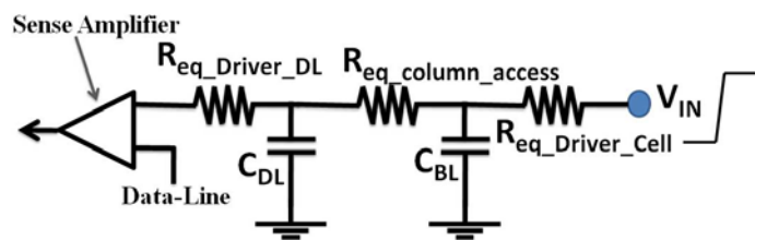
(c) RC Network During Read Operation
