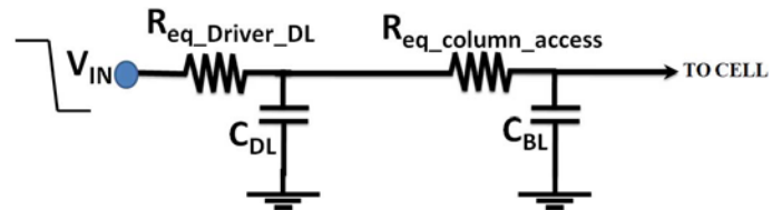
(b) RC Network During Write Operation
