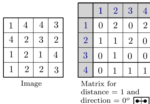
Fig. 6. Example of the co-occurrence matrix in the image.
