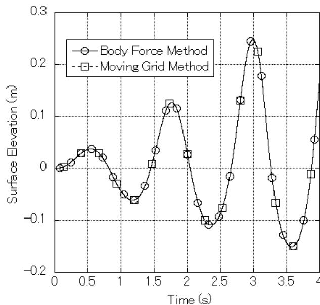
Fig. 5 Effect of oscillation amplitude
