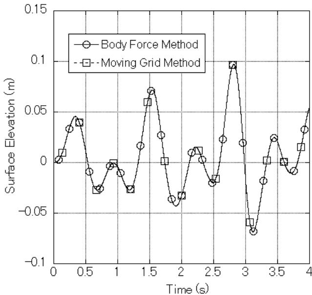
Fig. 6 Effect of oscillation frequency
